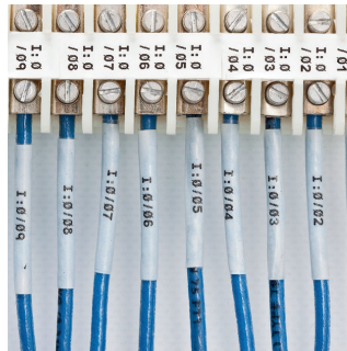
Heat Shrink Cable Labels
